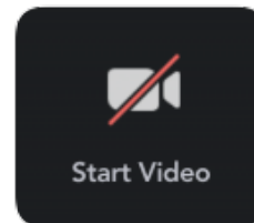
Start Video
