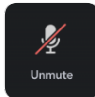
Unmute/Mute
